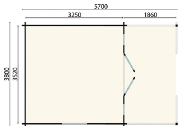
HANNA 2 floor plan
