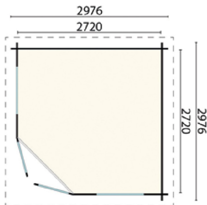
FLAT 280 floor plan
